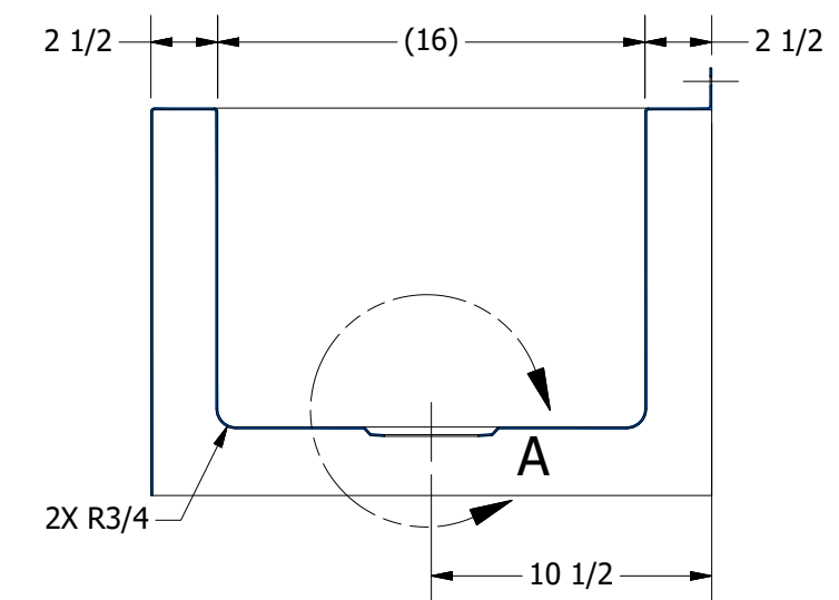
SECTION A-A SCALE 1/8
